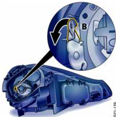
Halogen headlights
